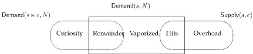
Figure 7. Demand/supply classes.
