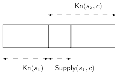
Figure 4. \text{SubAbsorber}(s_1, s_2) .
